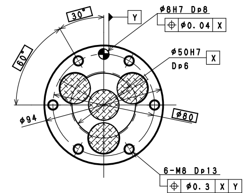
VIEW A
