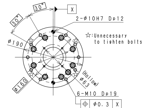
STANDARD FLANGE
