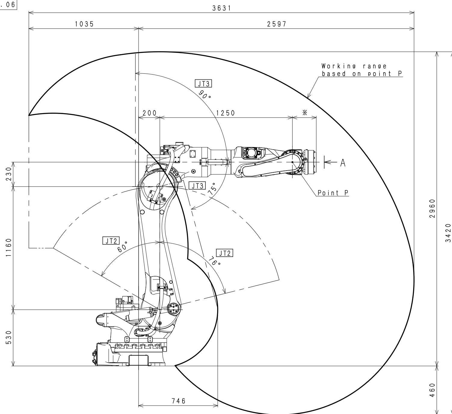
Installation Dimensions
