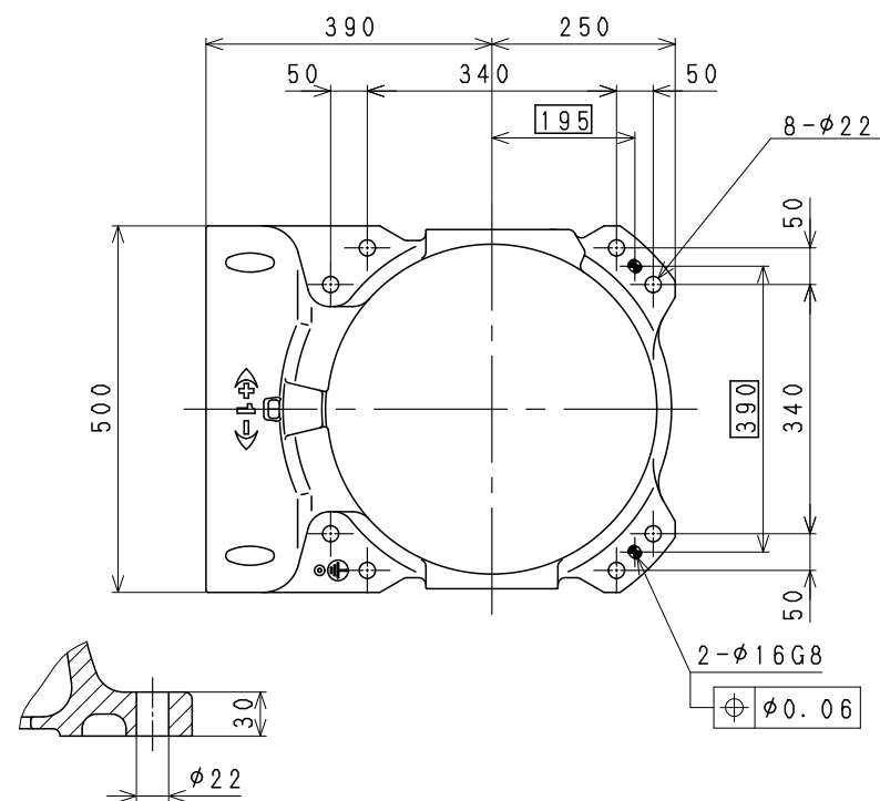
Installation Dimensions
