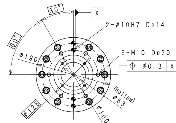
OPTION FLANGE
