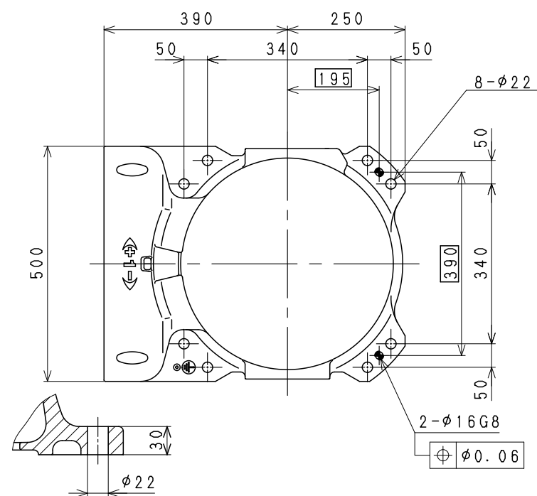
Installation Dimensions
