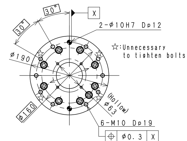
STANDARD FLANGE
