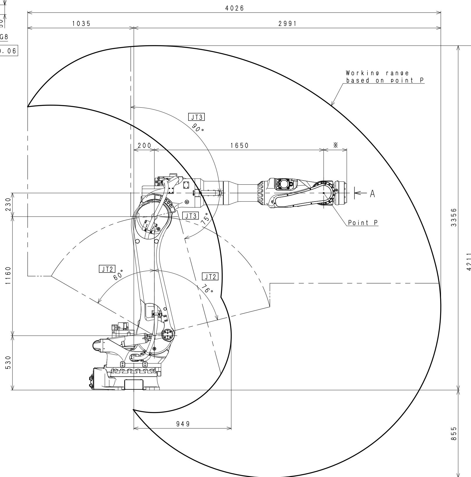
Installation Dimensions
